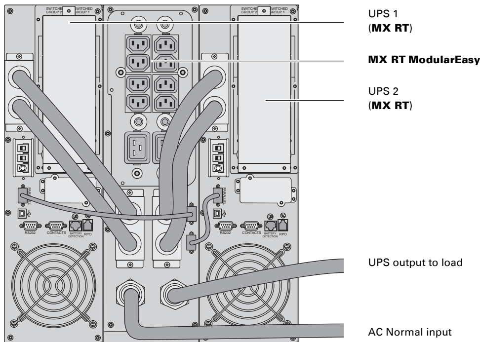
Example of MX ModularEasy connected with two UPSs in parallel operation
